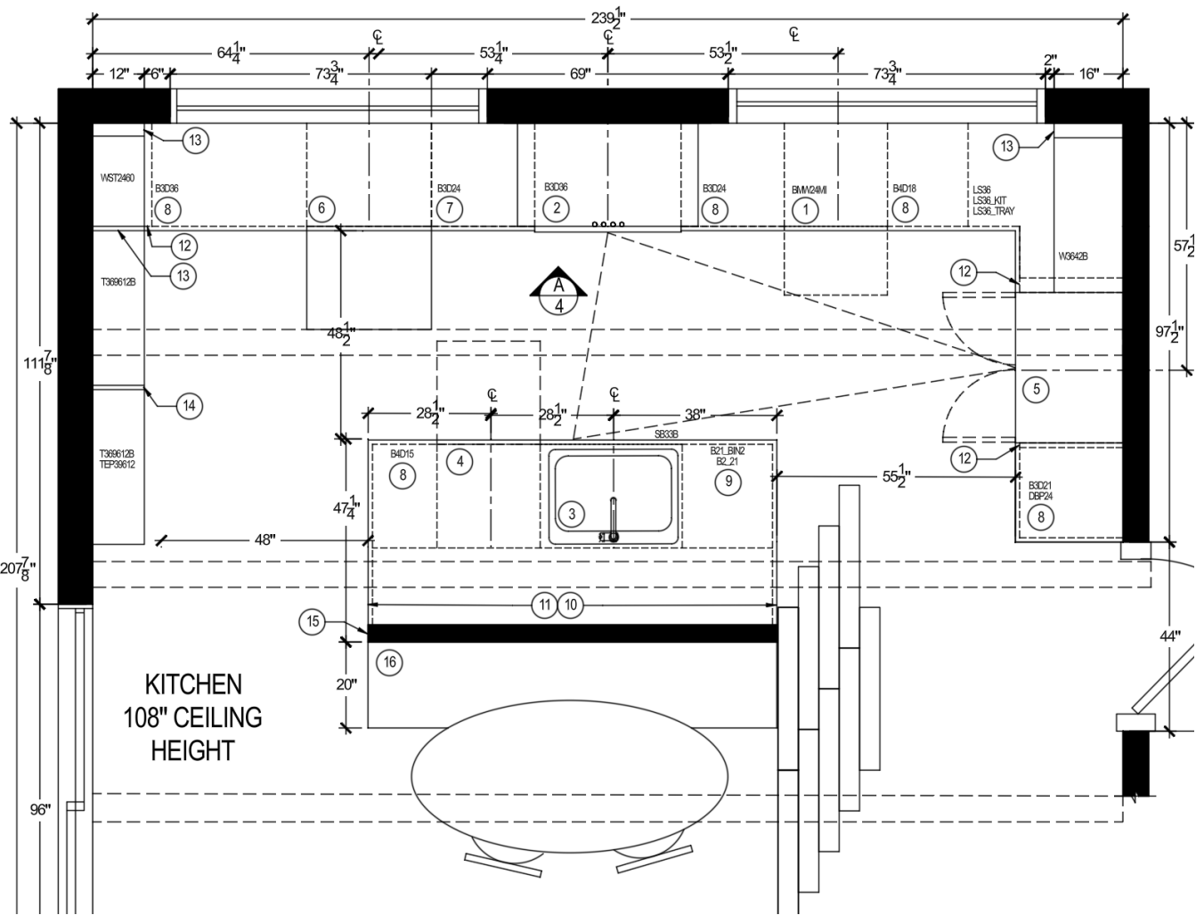
FLOOR PLAN
