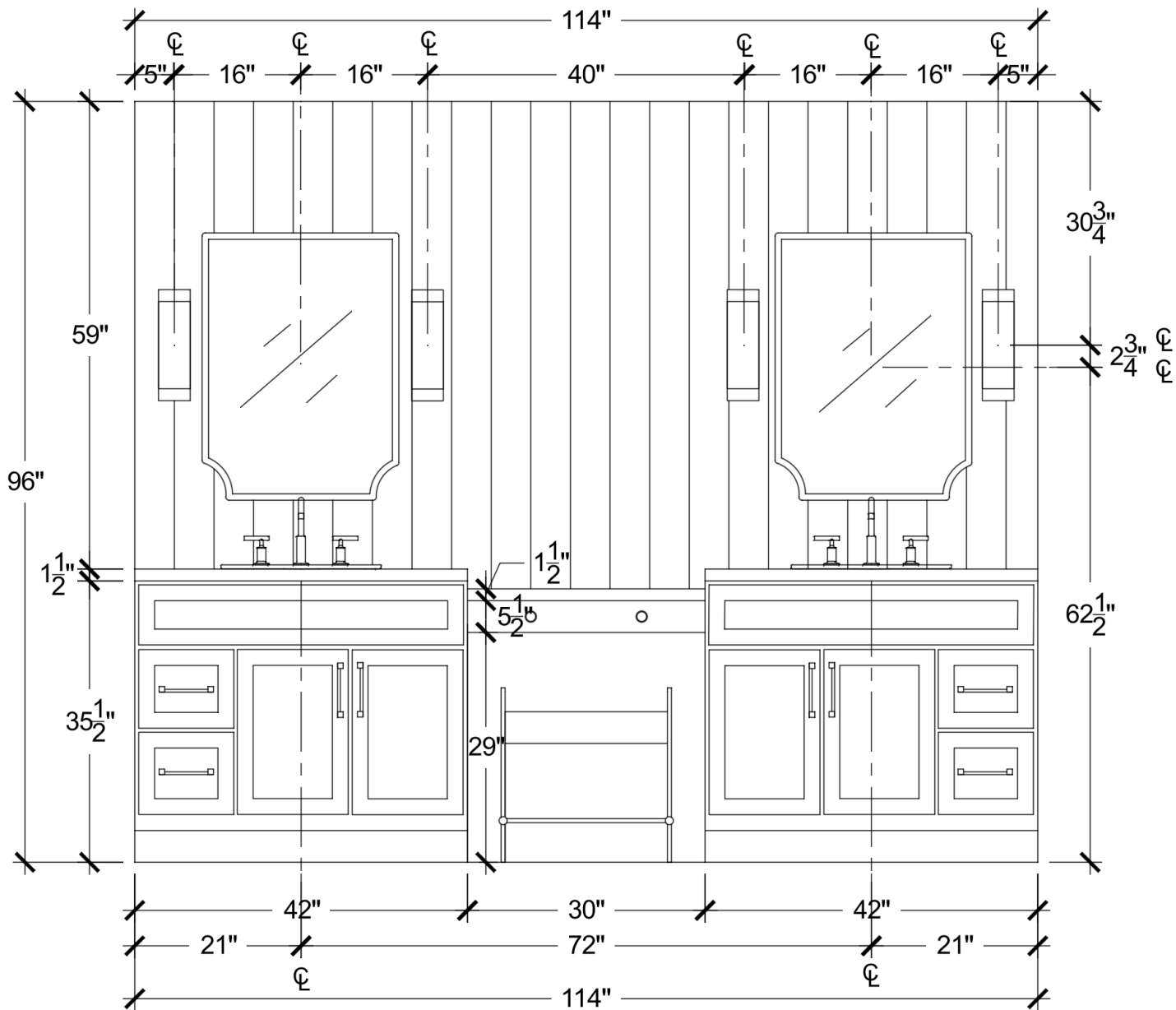
EAST ELEVATION
