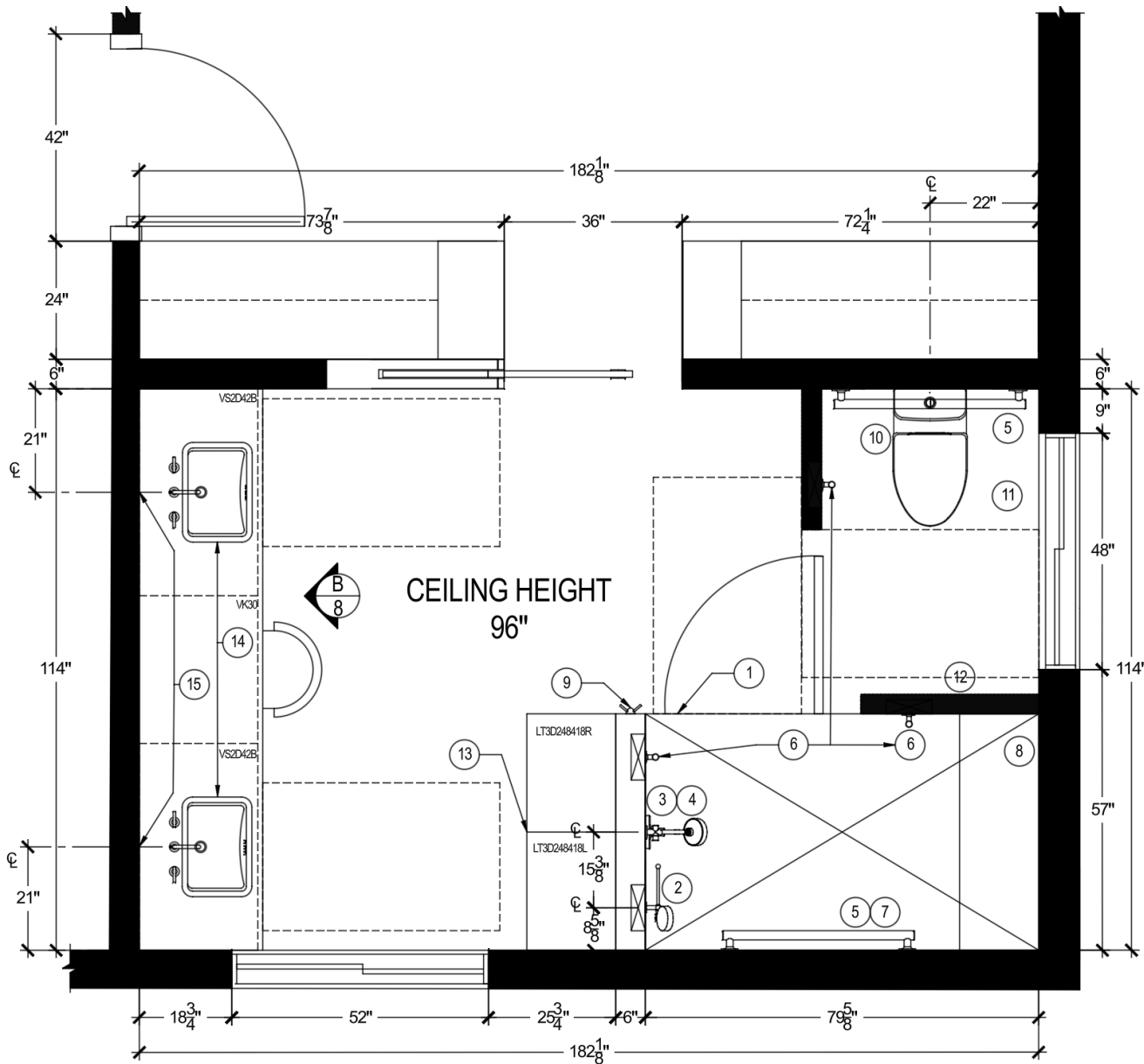
FLOOR PLAN
