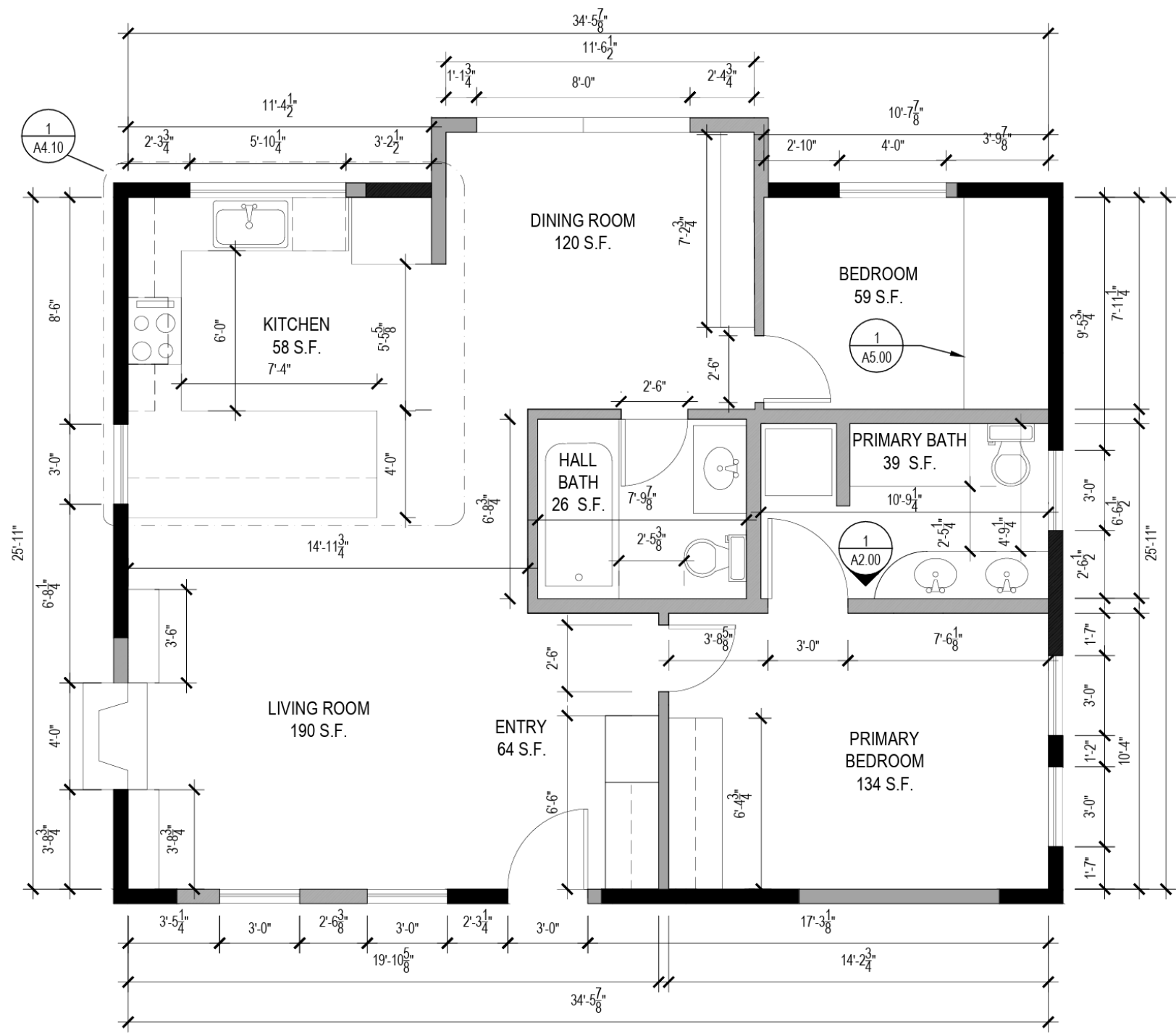
CONSTRUCTION PLAN
