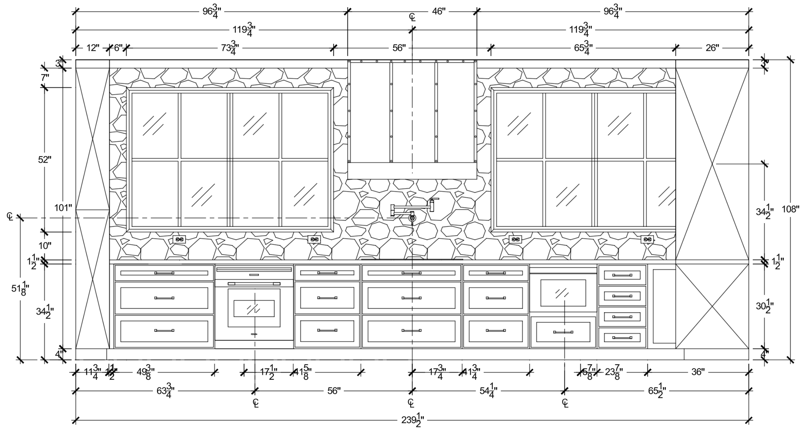
WEST ELEVATION
