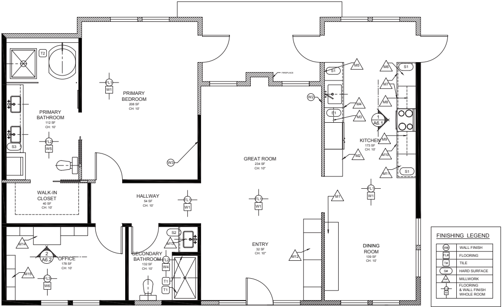
N FINISH FLOOR PLAN SCALE: 1/4" = 1'-0"
