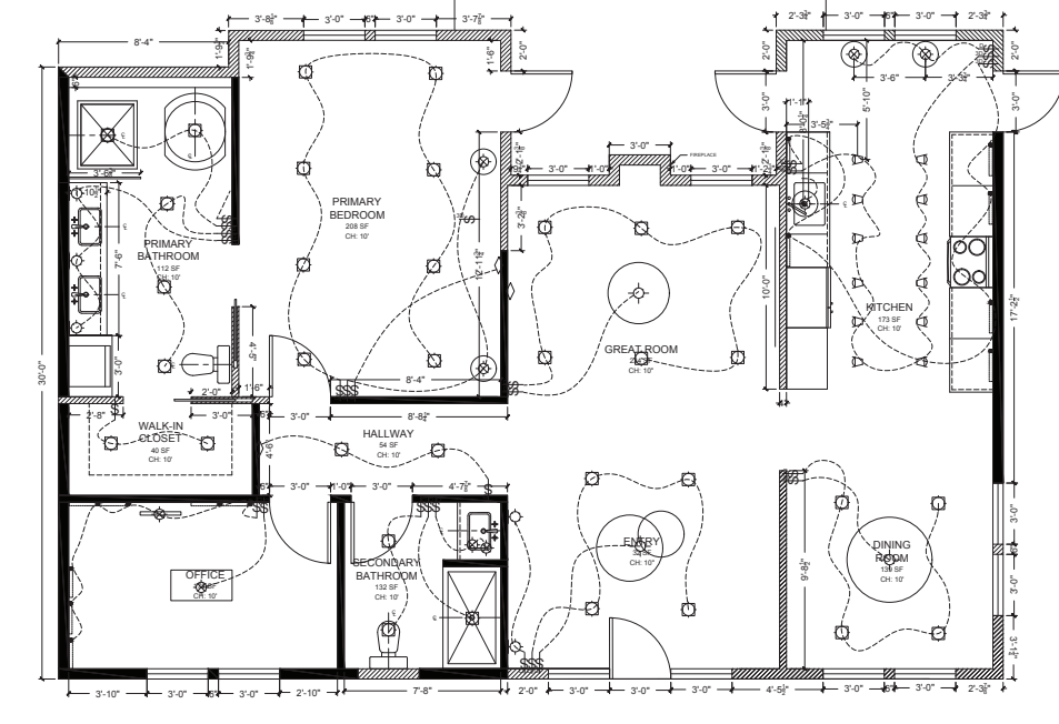
N LIGHTING PLAN SCALE: 1/4" = 1'-0"
