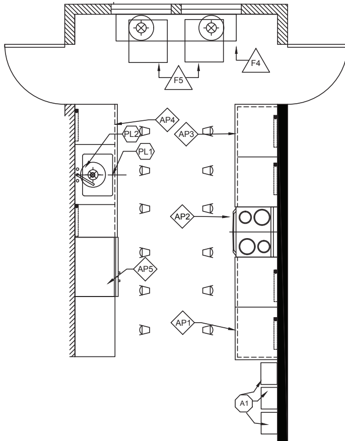
KITCHEN FLOOR PLAN
