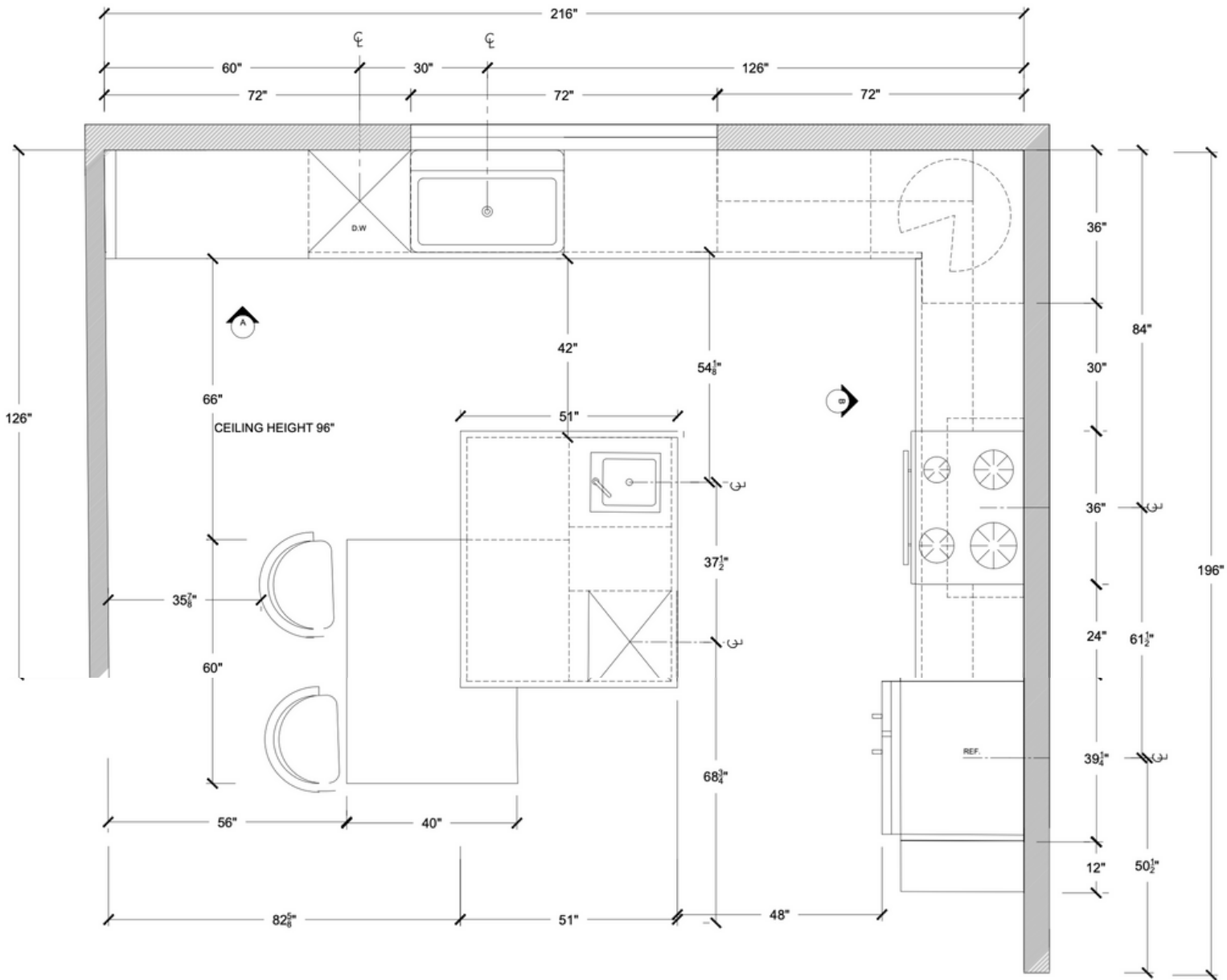
CONSTRUCTION PLAN AUTO CAD
