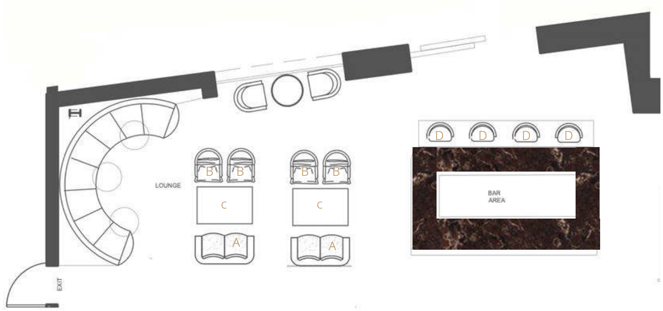
ENLARGED PLAN AUTO CAD
