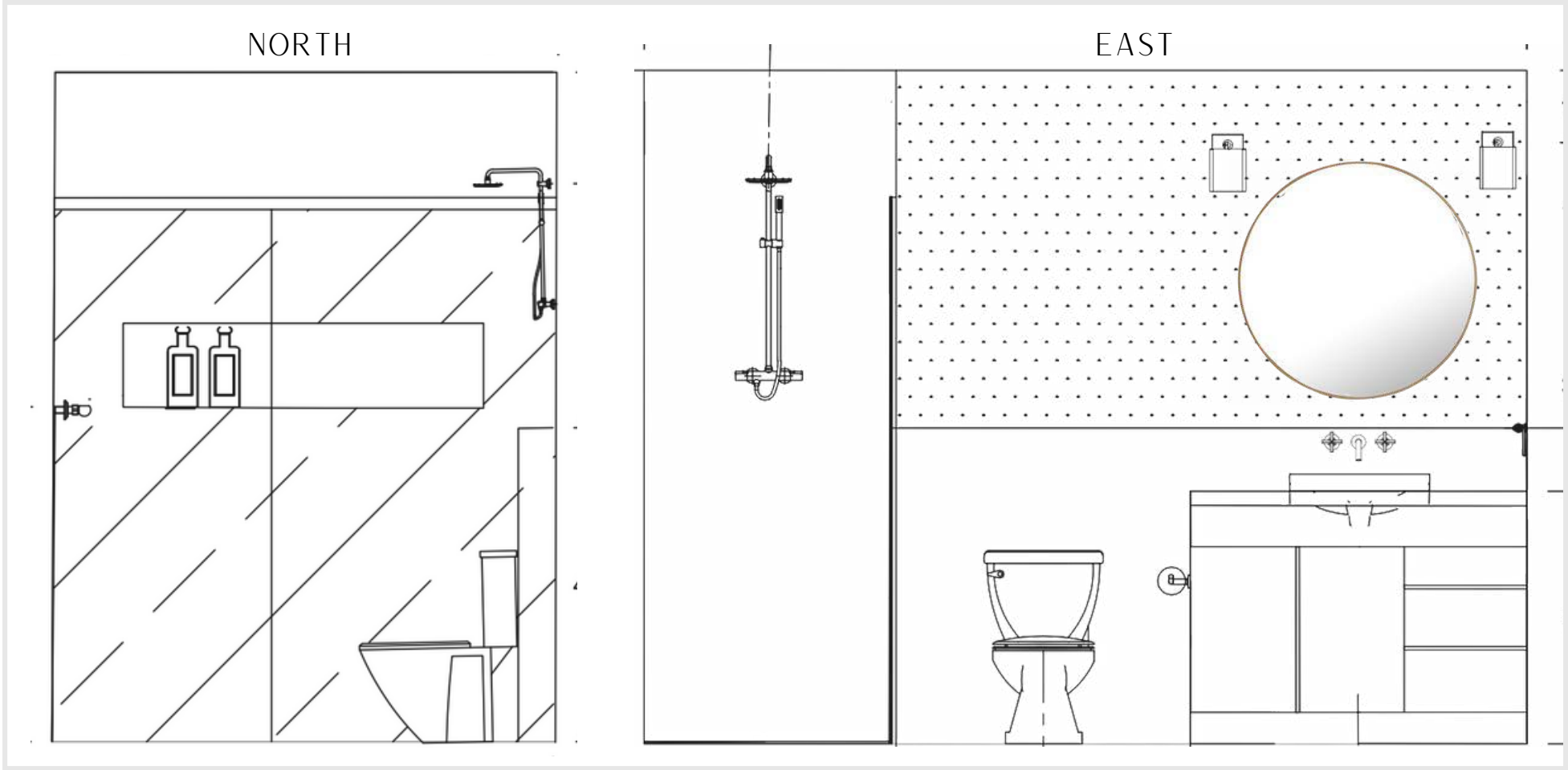
BATHROOM ELEVATION AUTO CAD
