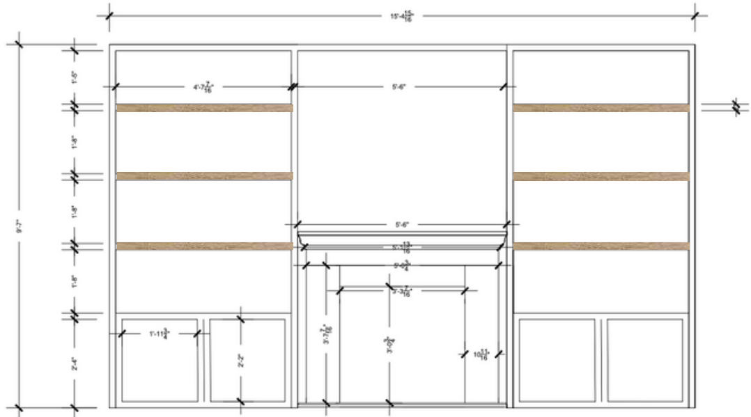
FIRE PLACE ELEVATION AUTO CAD
