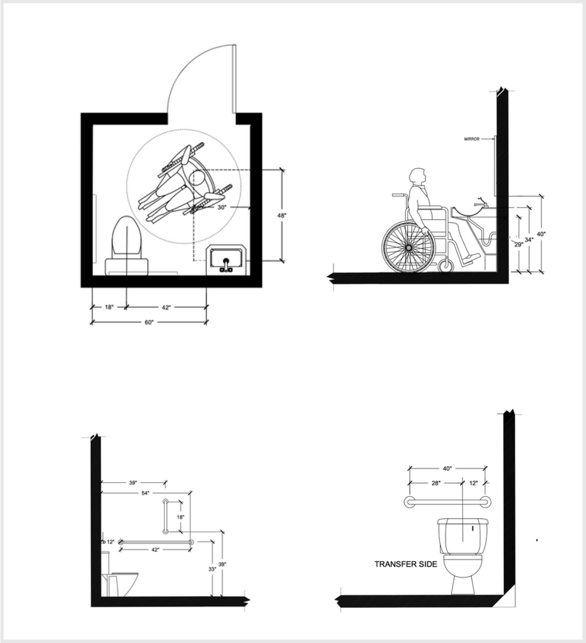
ADA BATHROOM ELEVATION AUTO CAD
