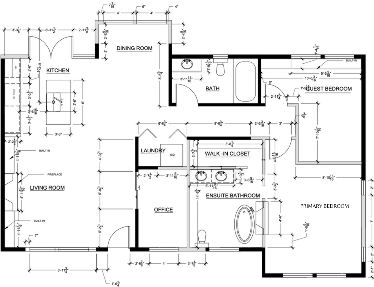
CONSTRUCTION PLAN AUTO CAD
