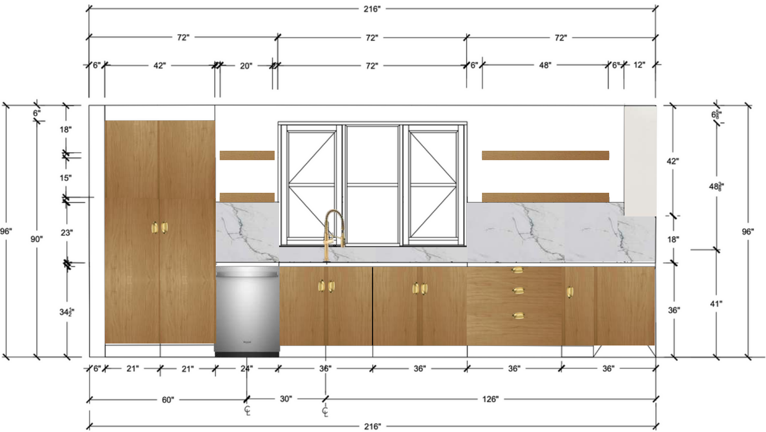
NORTH ELEVATION
