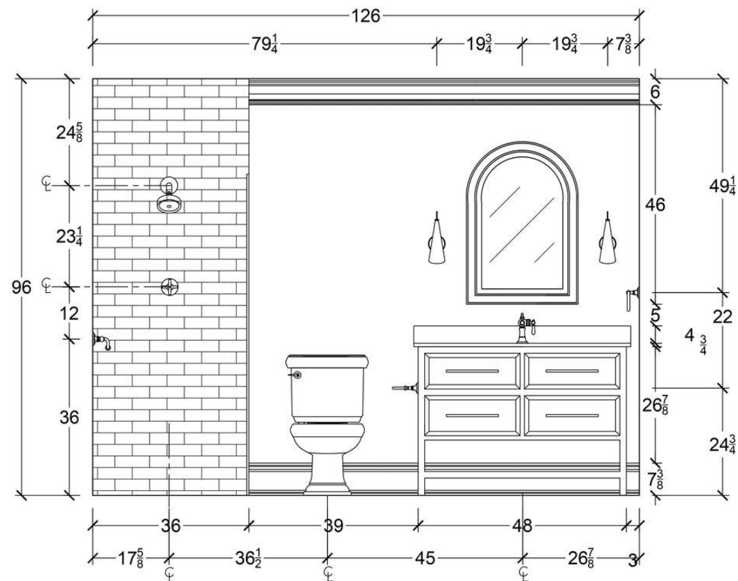
BATHROOM ELEVATIONS AUTOCAD
