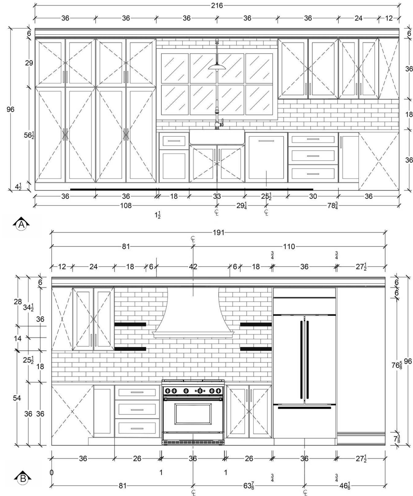
KITCHEN ELEVATIONS AUTOCAD
